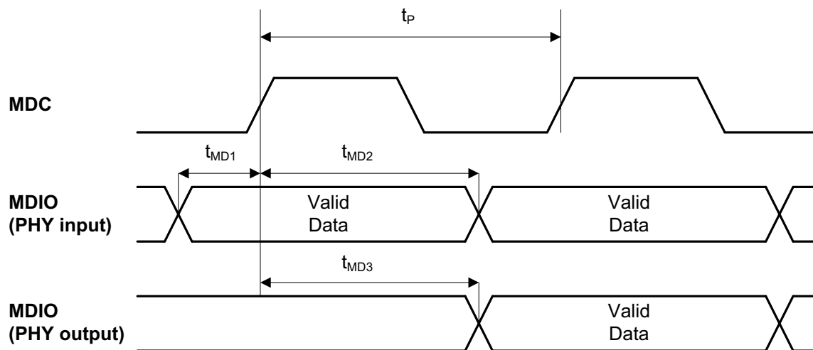
Figure 21. MDC/MDIO Timing
