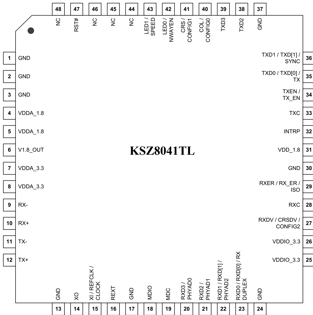
48-Pin TQFP
