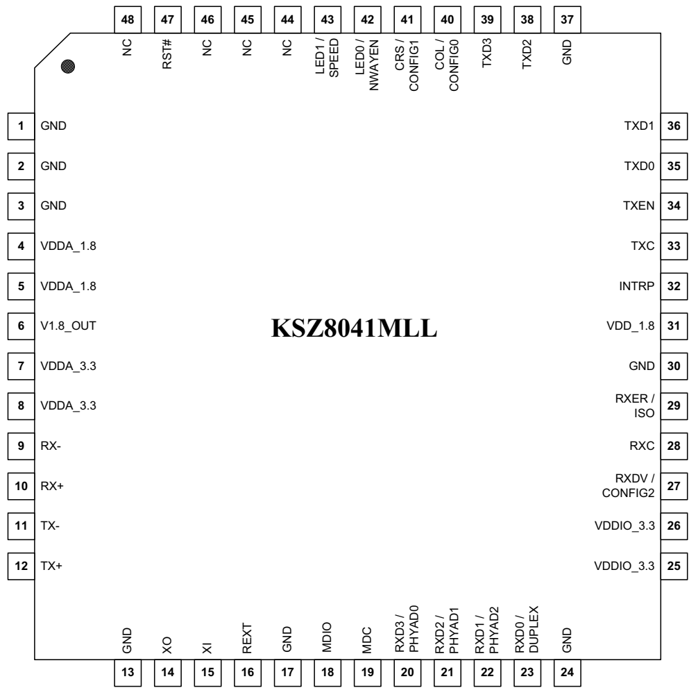
48-Pin LQFP
