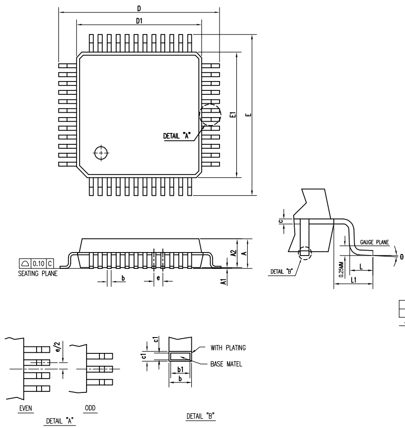
48-Pin (7mm x 7mm) LQFP Package
