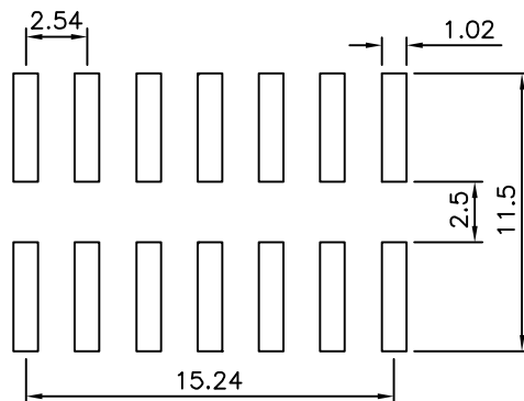
Recommended P.C.B. Layout PCB Tolerance:±0.05 (Top View)
