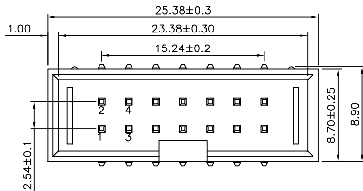
Recommended P.C.B. Layout PCB Tolerance:±0.05 (Top View)
